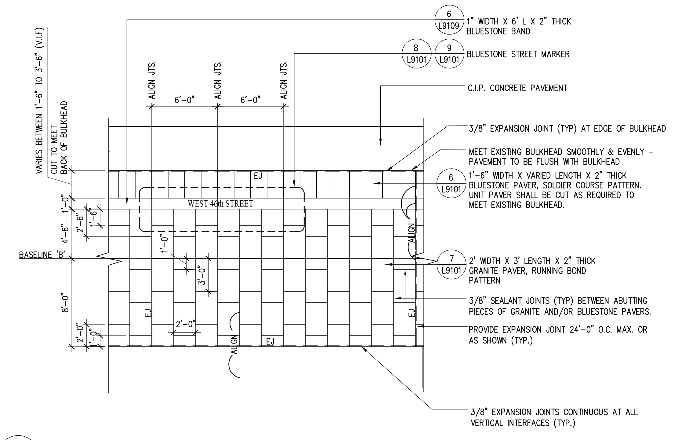
4 TYPICAL STREET MARKER PLAN/SECTION SCALE: 3/16"=1'-0"
