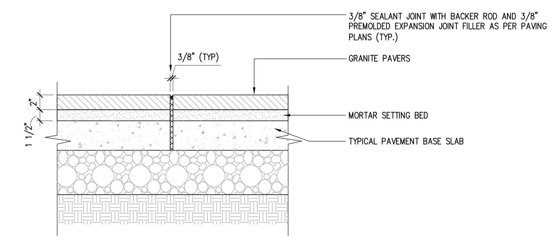
2 TYPICAL ESPLANADE PAVEMENT SCALE: 1 1/2"=1'-0"
