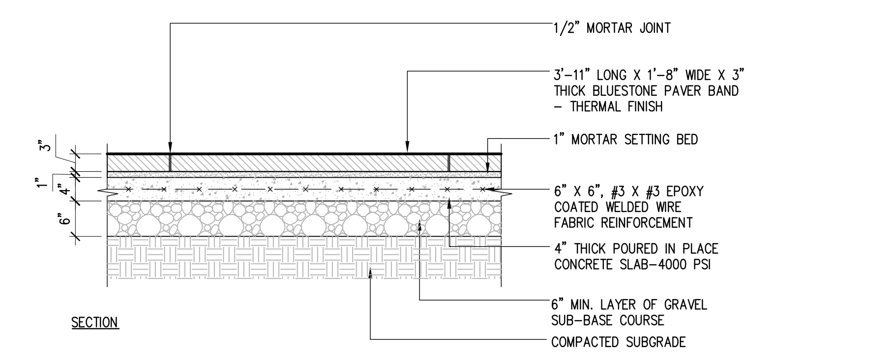
3 TYPICAL BLUESTONE PAVEMENT SCALE: 1 1/2"=1'-0"
